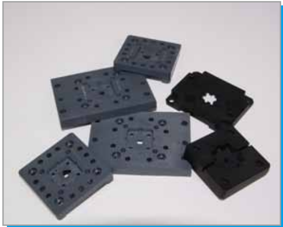
Figure 12. End Test Sockets made of Arylmax® K ESD Products
