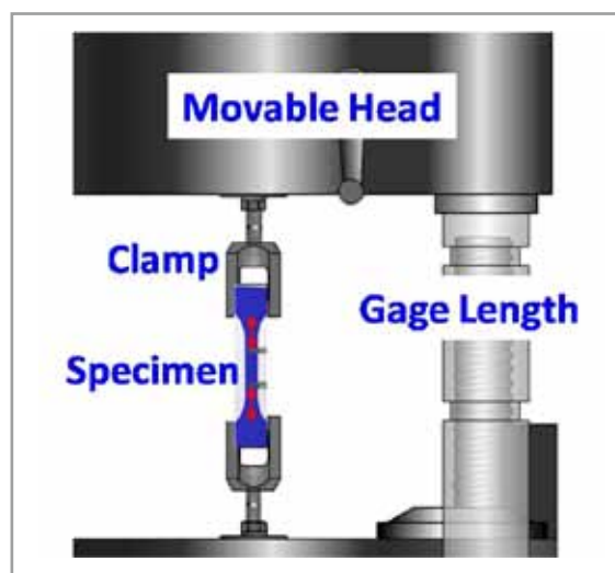
Figure 6. Tensile Properties Testing Diagram of Arylmax® K
