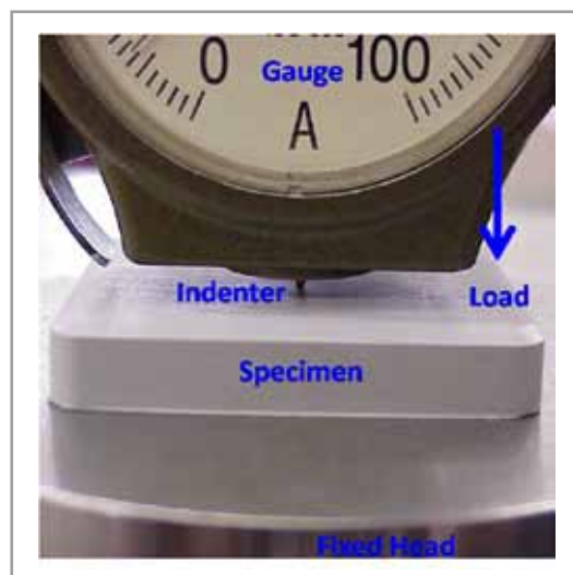
Figure 11. Hardness Properties Testing Diagram of Arylmax® K
