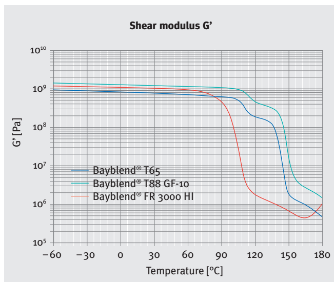
Fig. 5: Shear modulus G' from Bayblend® T65, T88 GF-10 and FR 3000 HI
