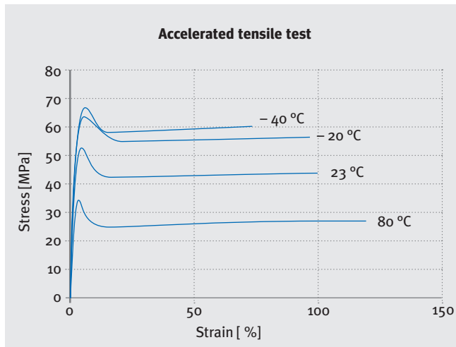
Fig. 1: Temperature-dependent stress-strain diagram for Bayblend T65 according to ISO 527-1,-2
