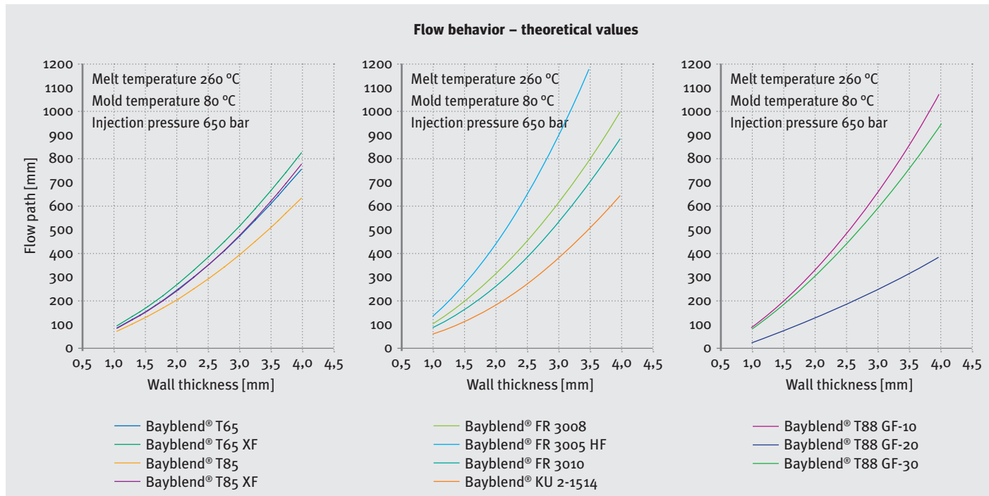
Figs. 6 to 8: Flow path/wall thickness diagrams
