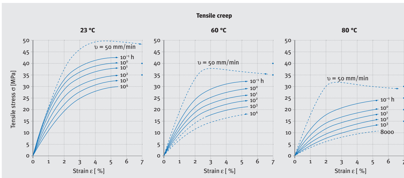
Figs. 2 to 4: Tensile creep according to DIN 53444 at various temperatures. Isochronous stress-strain curves. Bayblend® general-purpose grade Vicat 120 °C
