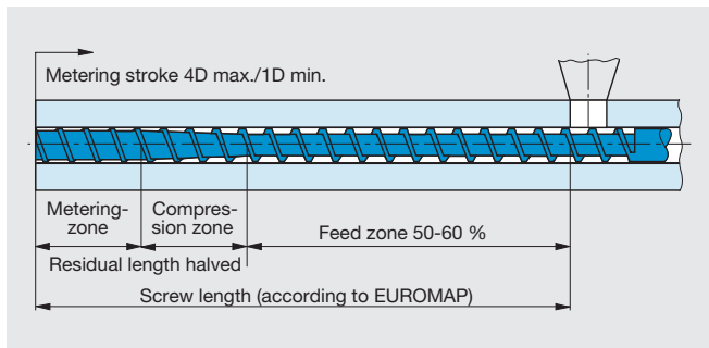
Fig. 12: Three-zone screw
